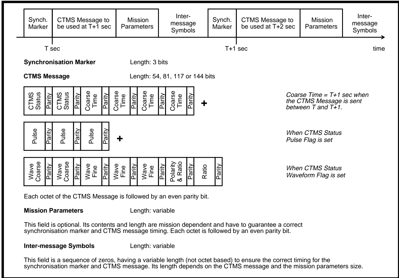
Figure 1.12 - Serial Protocol
