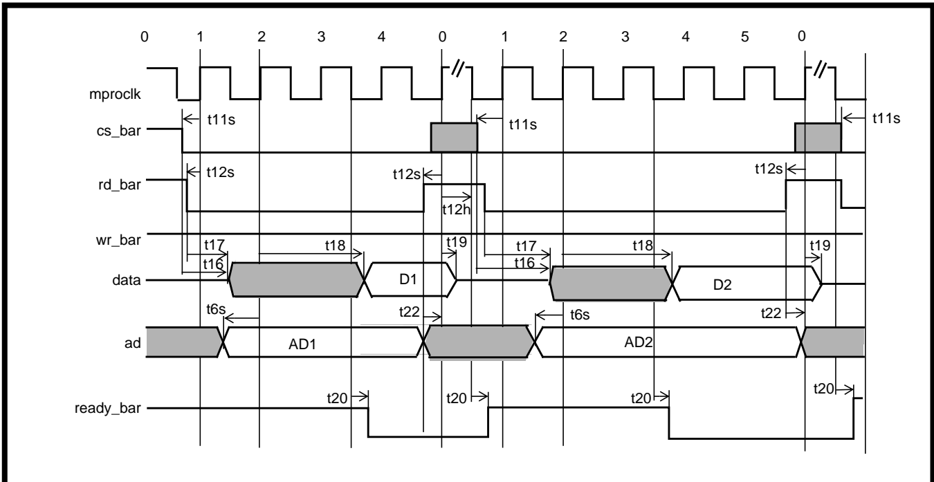
Figure 1.32 - MA31750 Read Cycle
