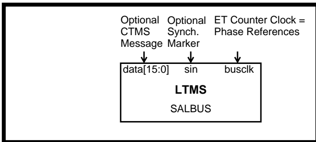
Figure 1.10 - SALBUS Operation
