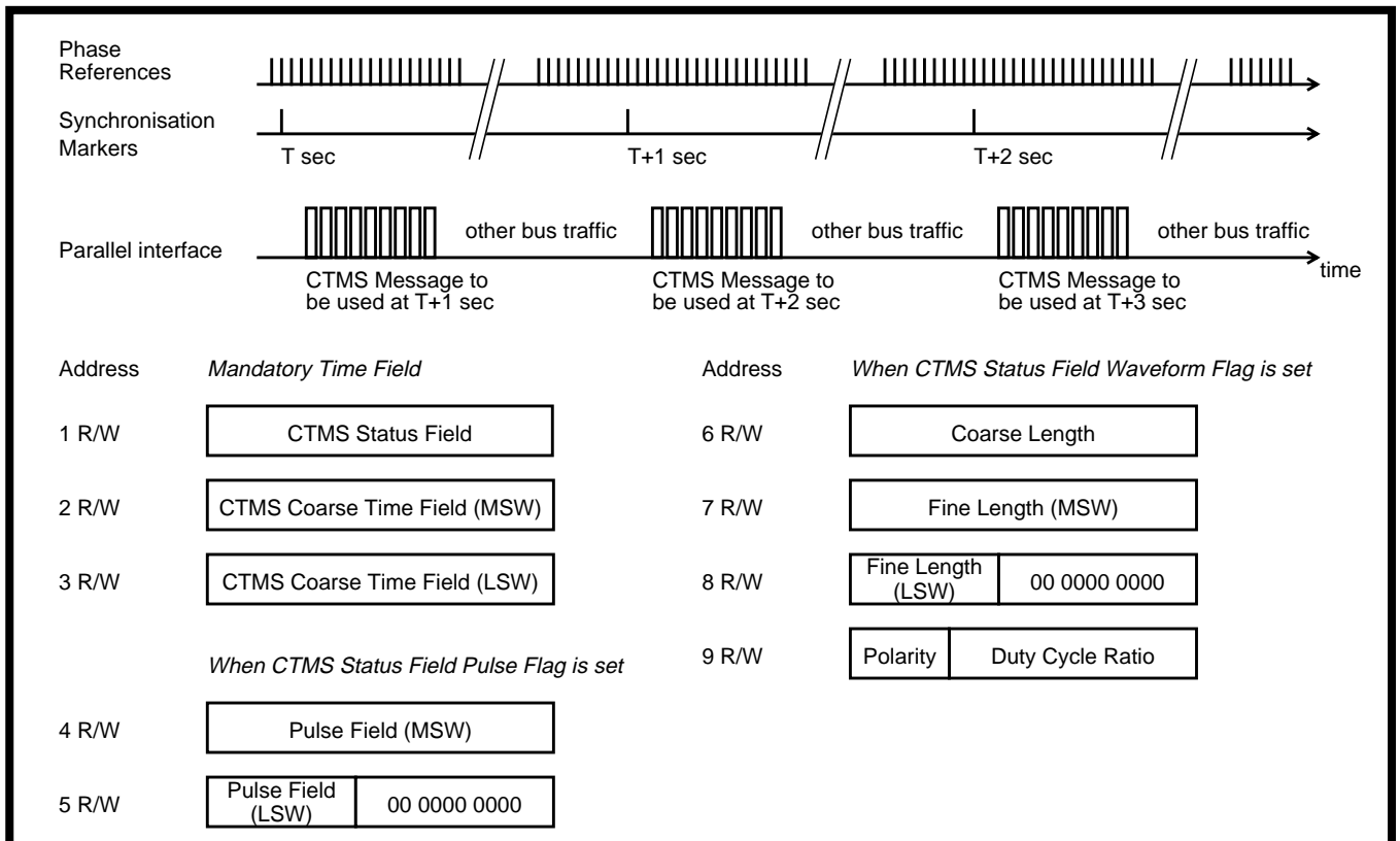
Figure 1.15 - Parallel Protocol
