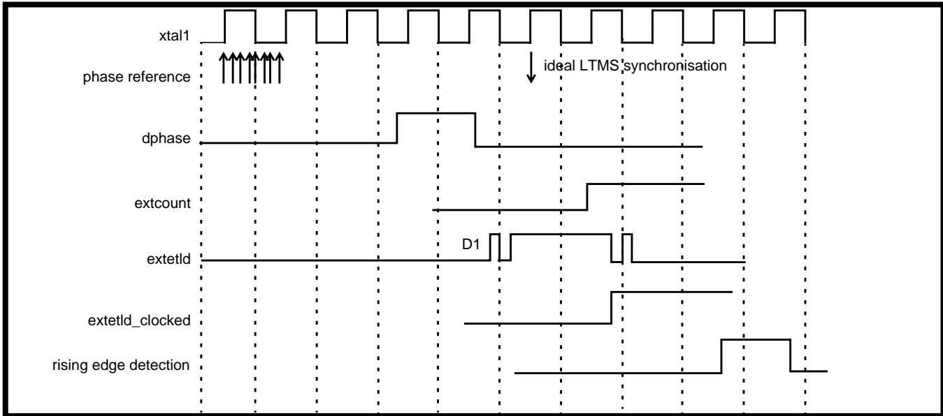
Figure B.1 - External DPLL Interface Usage
