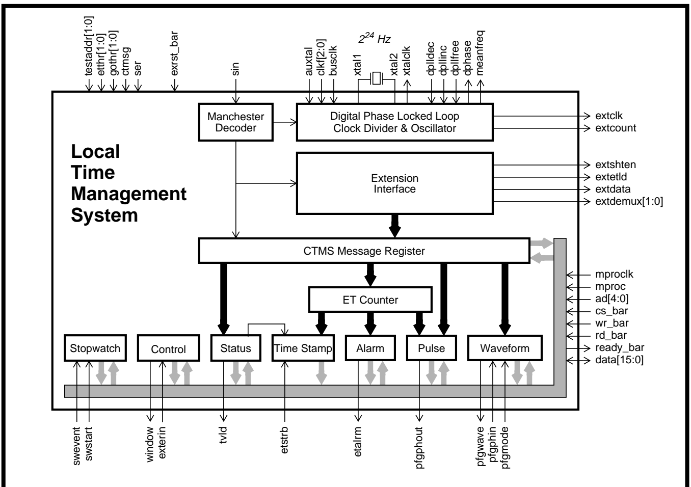
Figure 1 - LTMS Functional Block Diagram
