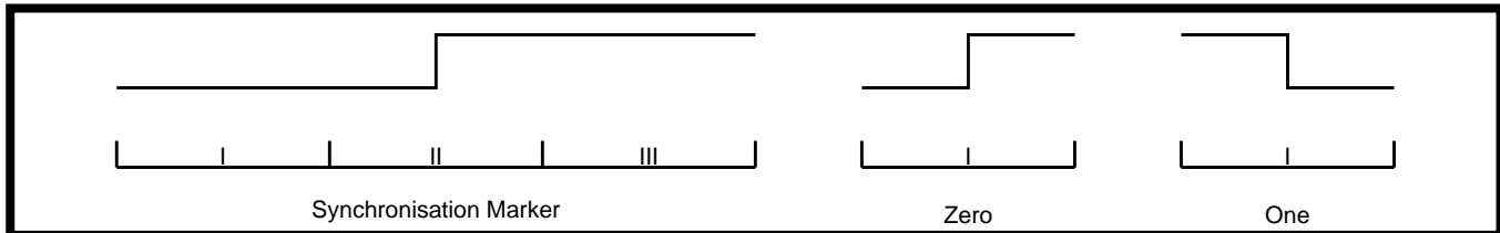
Figure 1.13 - Manchester Code
