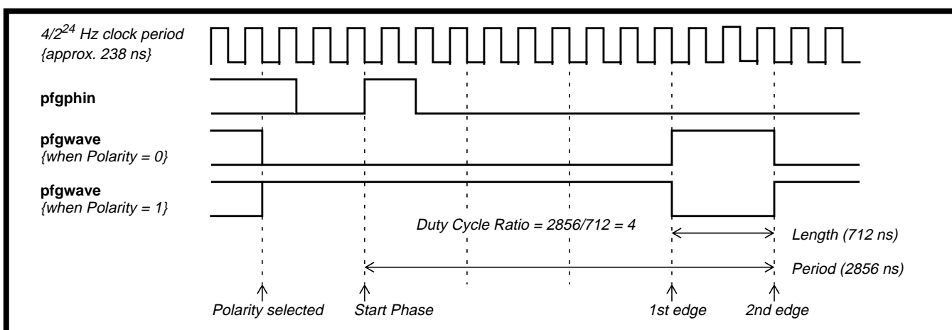
Figure 1.23 - Waveform Generator Facility Parameter Interpretation - an Example
