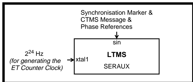
Figure 1.5 - SERAUX Operation
