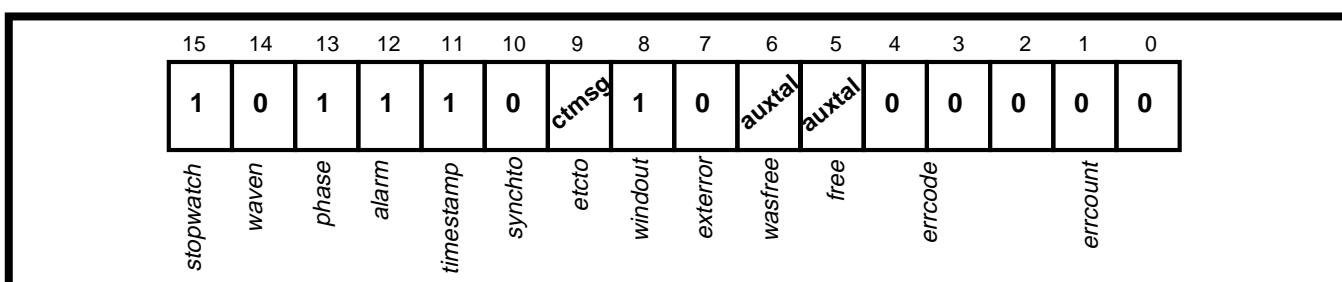
Figure 1.33 - LTMS Status Register - Initial Values
