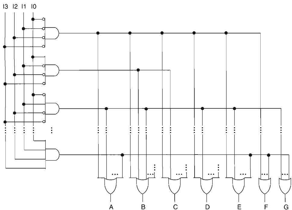
Figure 2-18. 7segment.gdf
