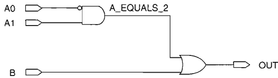
Figure 2-11. boole2.gdf
