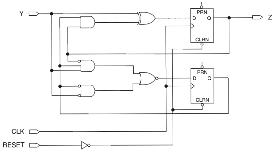
Figure 2-43. moore1.gdf
