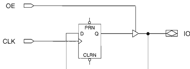
Figure 2-27. bus_reg2.gdf
