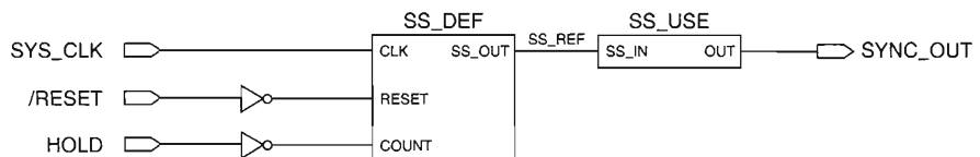
Figure 2-57. top1.gdf
