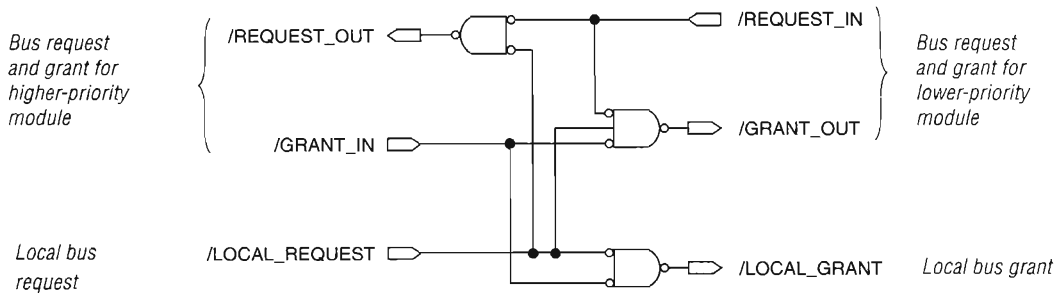
Figure 2-25. daisy.gdf
