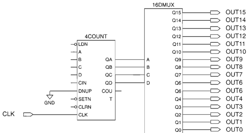
Figure 2-51. macro.gdf
